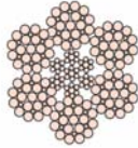
ROUND STRAND 6/19F (12-6F+6-1) Page # 81
