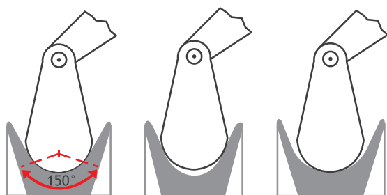
Figure 57 Grooves inspection: correct size, narrow and large groove
