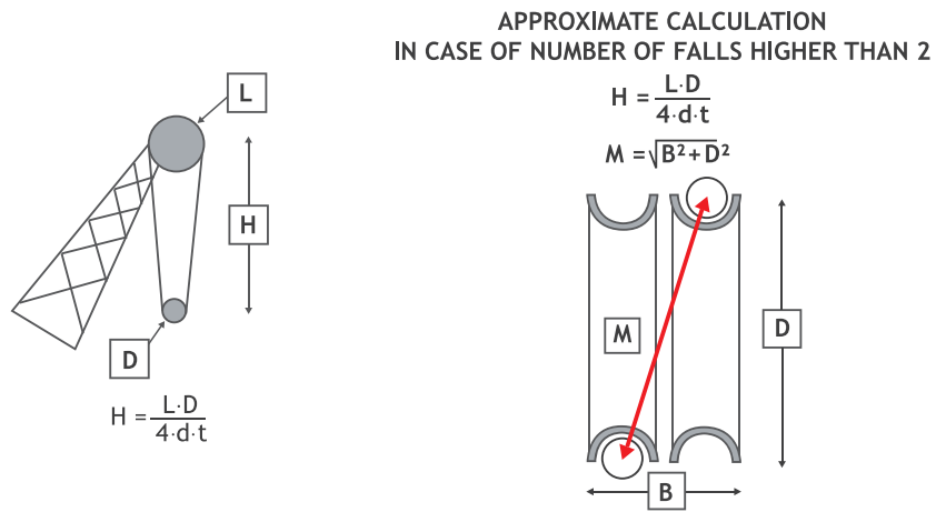
Figure 23 Calculation of maximum lifting height
