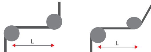
Figure 43 Reverse bending and partial reverse bending
