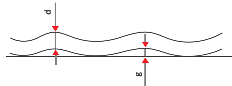
Figure 62 Waviness assessment
