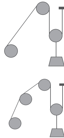
Figure 42 2 Falls with 2 rotating sheaves and with an extra sheave
