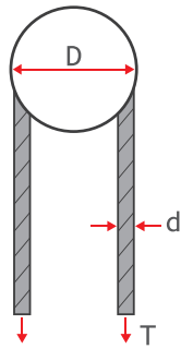
Figure 46 Rope pressure over a sheave
