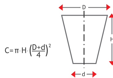
Figure 37 Resin content and cone dimensions
