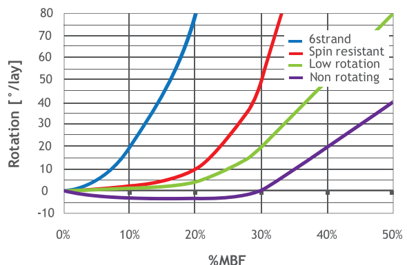
Figure 21 Rotation for different rope constructions
