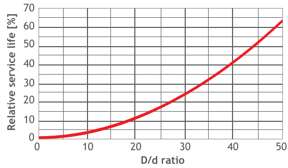
Figure 52 Effect of bending ratio on service life
