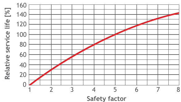
Figure 50 Effect of safety factor on service life
