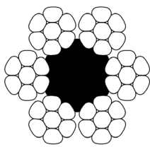
6xK7 - FC
