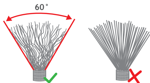
Figure 36 Socket brush
