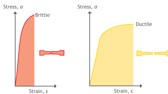
Figure 7 Stress - strain curves
