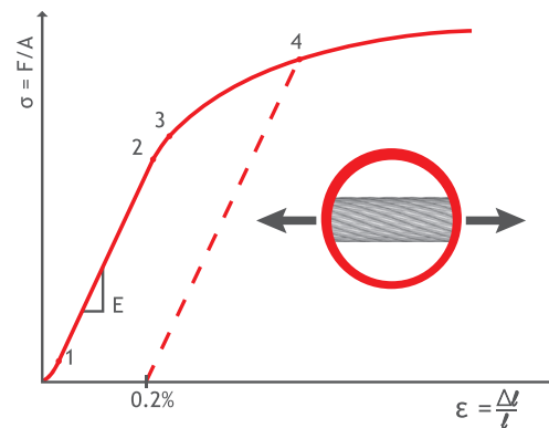
Figure 17 Stress - strain curve for a wire rope
