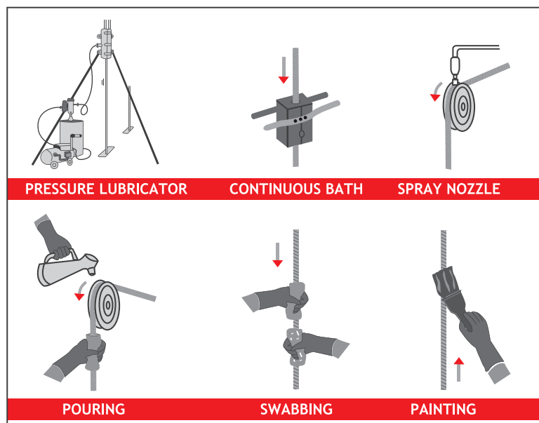
Figure 49 Typical lubrication modes
