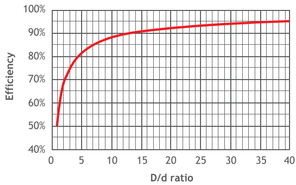
Figure 40 Reduction in rope efficiency in case of bent over stationary components
