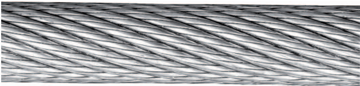
Figure 26 Example of rope with very low outer lubrication
