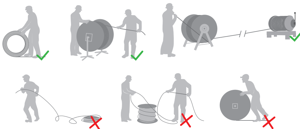
Figure 33 Recommendations for rope pay out
