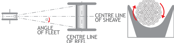
Figure 13 Fleet angle during spooling and rope rolling
