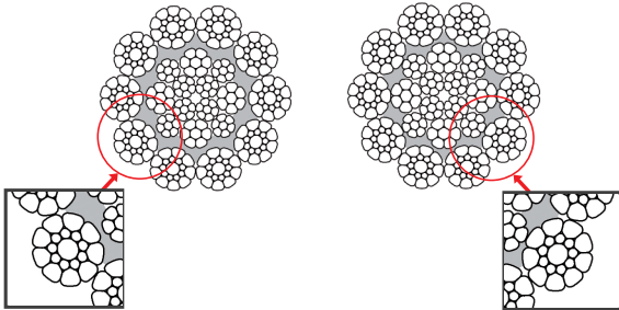
Figure 16 Cushion layer versus plastic impregnated core
