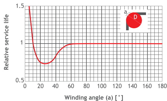
Figure 45 Relative service life depending on winding angle
