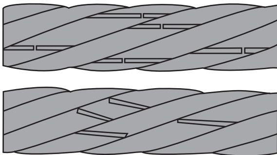
Figure 60 Crown and valley breaks due to fatigue
