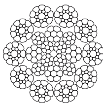
10xK19S - IWRC
