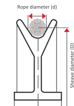
Figure 58 Bending ratio between rope and sheave
