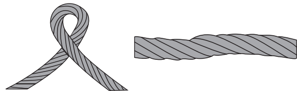
Figure 32 Rope kink and associated deformation
