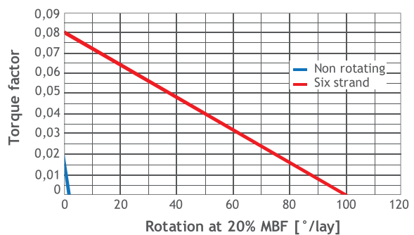
Figure 20 Torque factor for non rotating and six strand ropes
