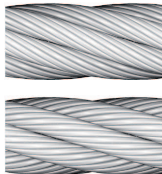
Figure 5 Lang lay (first figure) and regular lay (second figure)
