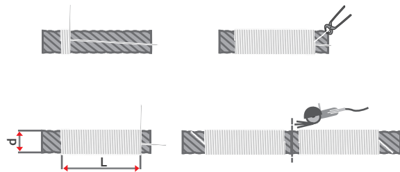
Figure 30 Serving dimensions and configuration
