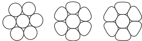
Figure 10 Round strand, light and high compacting level
