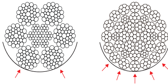
Figure 47 Pressure distribution of 6 strand and non rotating rope
