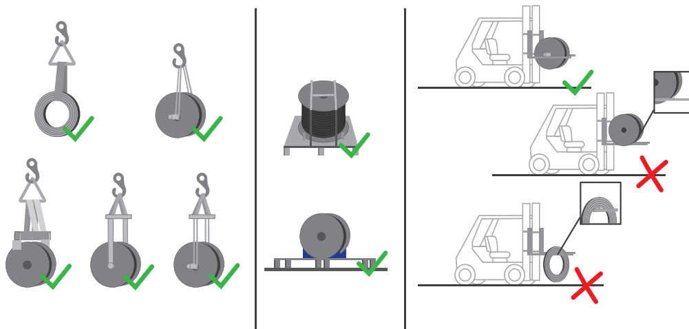
Figure 28 Rope handling recommendations
