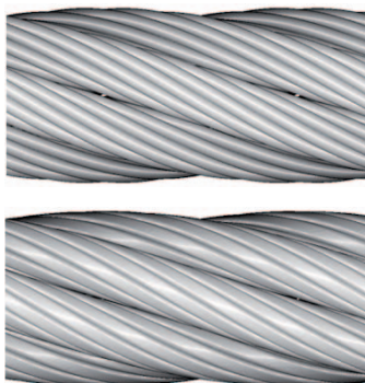
Figure 11 Round strand versus compacted strand
