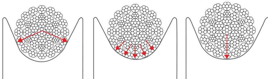
Figure 48 Pressure distribution for narrow, well dimensioned and large grooves
