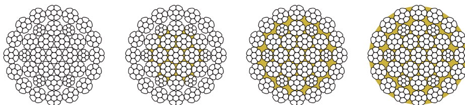
Figure 27 Typical lubrication levels
