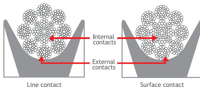
Figure 12 Contact surfaces for a non compacted and a compacted rope
