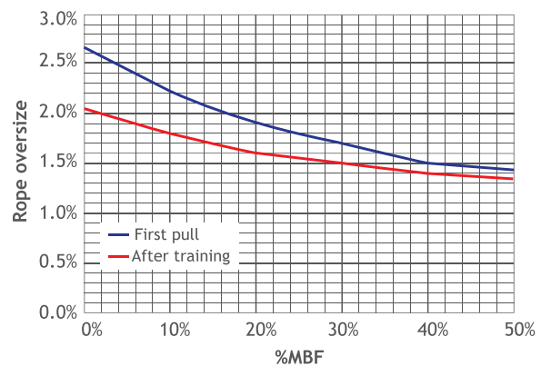
Figure 18 Rope oversize versus load
