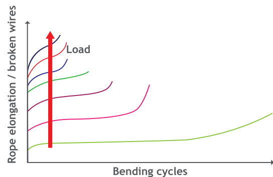
Figure 51 Fatigue progression
