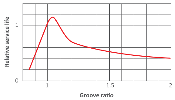
Figure 54 Effect of groove ratio on service life
