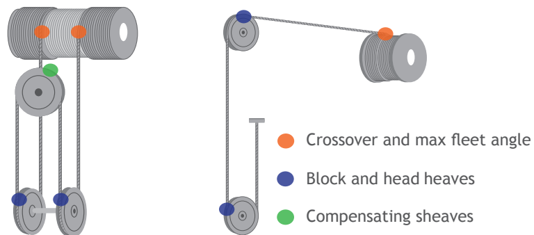
Figure 56 Areas requiring detailed inspection
