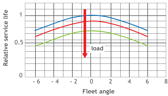
Figure 53 Effect of fleet angle on service life
